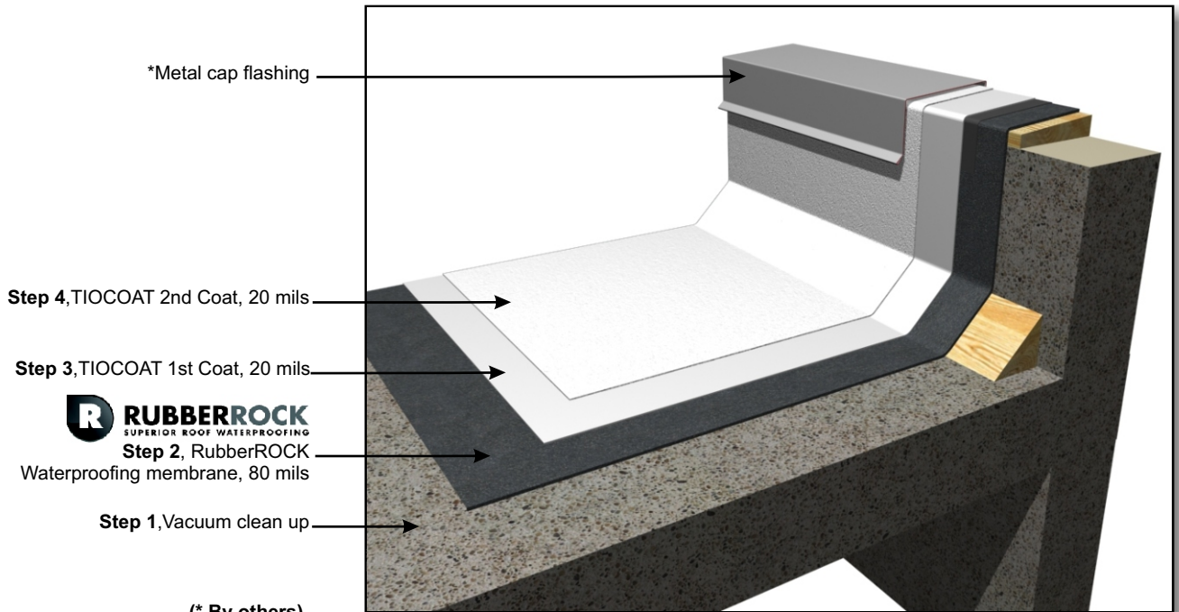
CONCRETE ROOF AFTER SYSTEM APPLICATION
